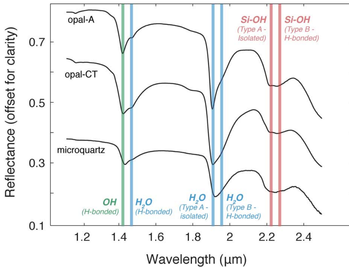
Figure 1.2 — Near-infrared spectra of varieties of hydrated silica (spectra courtesy of E. Cloutis, University of Winnipeg). Absorption bands are labeled with their causal molecule. Further information on vibrational modes is given in Table 1.3 .
