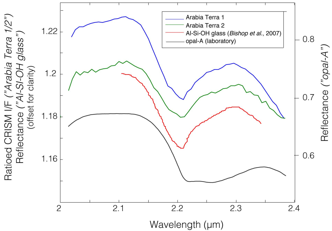
Figure A.1 - Comparison of 2.2 \mu\text{m} Si-OH feature from Arabia Terra relative to laboratory samples. The shape of Martian spectra are not a good match for hydrated silica, but are a better match with amorphous Al-Si-OH glass from Haleakala, Maui, Hawaii [Bishop et al. 2007].
