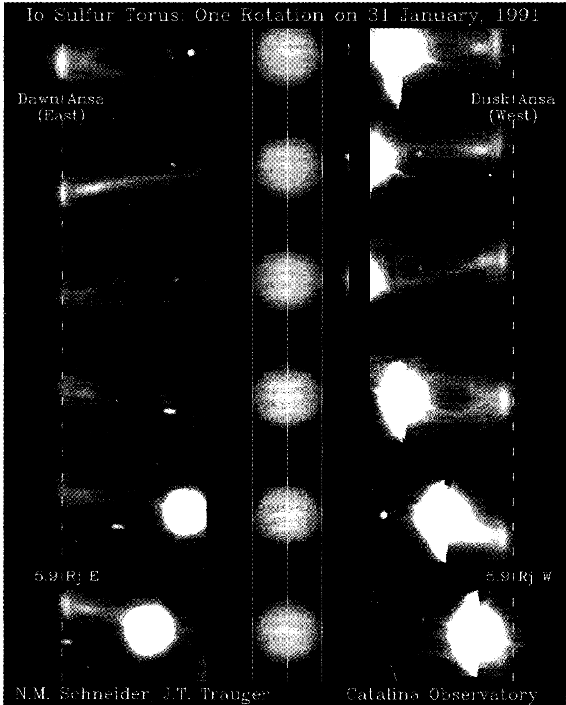
Figure 1.3: Io torus observed using sodium D line emissions from the Catalina Observatory [Schneider and Trauer, 1995].
