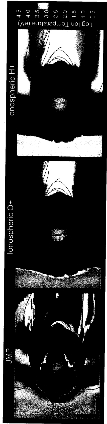
Figure 6.4: Discuss the energization of the various ion species, as well as precipitation as it pertains to the ionosphere and magnetospheric shielding.
