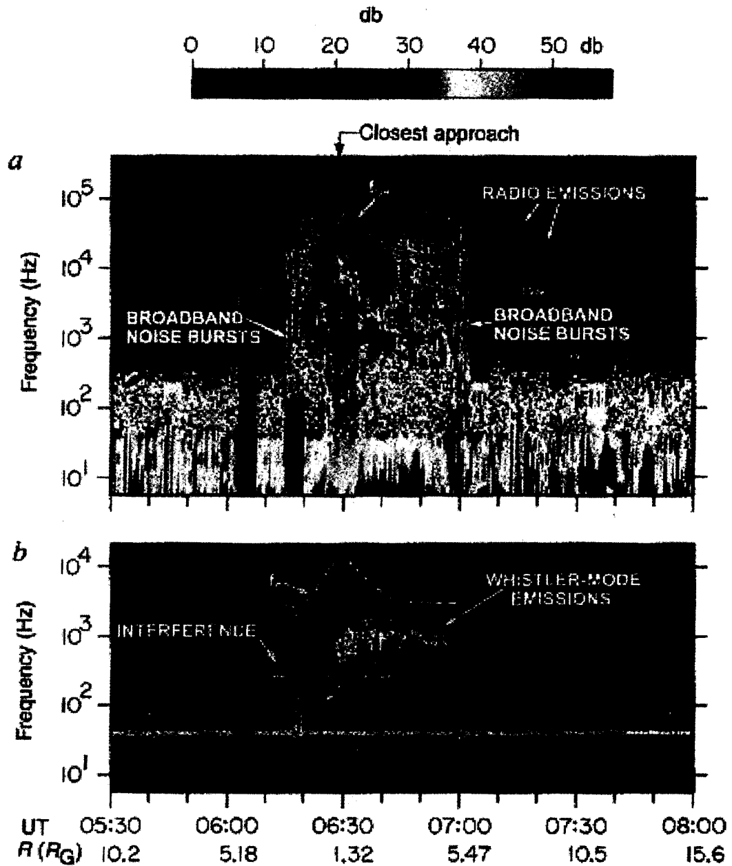
Figure 2.3: From Gurnett et al. [1996], the electric (a) and magnetic field (b) spectrograms.
