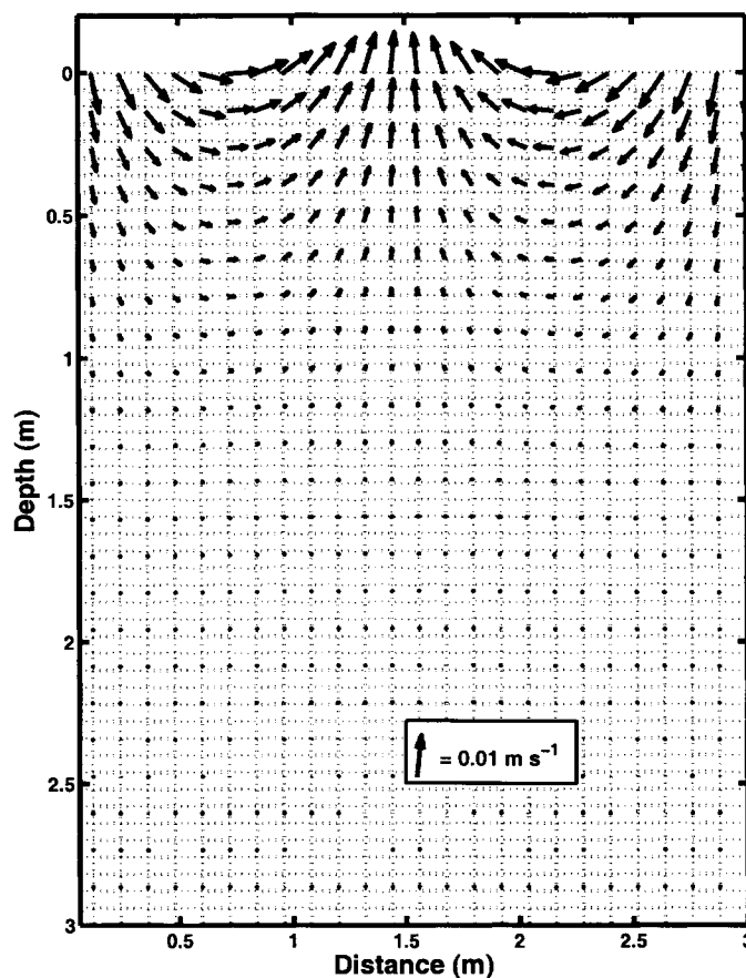
Figure 5.1: Air flow in the firn (ventilation) is the result of steady wind flow ( 10 \text{ m s}^{-1} ) over a sinusoidal surface topography (wavelength of surface topography = 3 \text{ m} , surface amplitude = 0.1 \text{ m} ). Air-flow velocity vectors are calculated as in Colbeck (1989) and Waddington and others (1996), and have a maximum value of 0.01 \text{ m s}^{-1} . Air flows into the firn between 0.75 \text{ m} and 2.25 \text{ m} in the horizontal direction, and out of the firn between 0 and 0.75 \text{ m} . Note that air-flow velocities are calculated on a rectangular grid, rather than along the actual sinusoidal snow surface. Cunningham and Waddington (1993) showed that this is a reasonable approximation as long as the aspect ratio of the bumps is < 1 .
