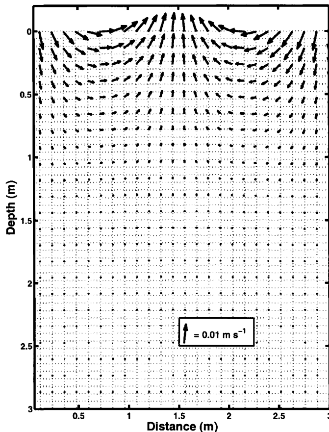
Figure 4.2: Air flow in the firn (ventilation) is the result of steady wind flow ( 10 \text{ m s}^{-1} ) over a sinusoidal surface topography (wavelength of surface topography = 3 \text{ m} , surface amplitude = 0.1 \text{ m} ). Air-flow velocity vectors are calculated as in Colbeck (1989) and Waddington and others (1996), and have a maximum value of 0.01 \text{ m s}^{-1} . Air flows into the firn between 0.75 \text{ m} and 2.25 \text{ m} in the horizontal direction, and out of the firn between 0 and 0.75 \text{ m} and 2.25 \text{ m} and 3 \text{ m} . Note that air-flow velocities are calculated on a rectangular grid, rather than along the actual sinusoidal snow surface. Cunningham and Waddington (1993) showed that this is a reasonable approximation as long as the aspect ratio of the bumps is < 1 .
