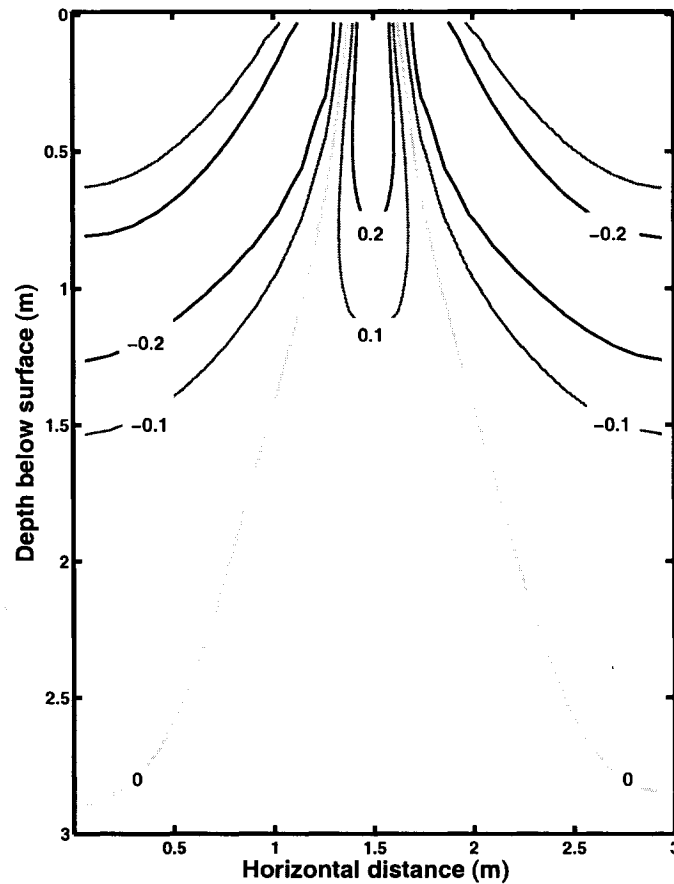
Figure 4.4: Contours of mass-transfer rate (given in 10^{-6} \text{ kg m}^{-3} \text{ s}^{-1} ) calculated using environmental conditions typical of Antarctic summer with sub-surface air flow as in Figure 4.2. Contours of 0, \pm 0.1 and \pm 0.2 \times 10^{-6} \text{ kg m}^{-3} \text{ s}^{-1} are plotted. Positive values indicate sublimation, negative values indicate condensation. Air flowing into the firn reaches saturation vapor pressure in the upper 0.05 m regardless of the initial relative humidity of the atmosphere (Chapter 3). Condensation in regions of inflowing air is a result of the advection of relatively warm and moist air from the atmosphere into progressively colder and drier regions. Regions of air outflow are marked by sublimation, as cold and dry air from the firn interior is advected into progressively warmer near-surface regions.
