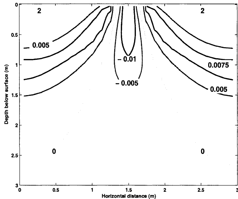
Figure 3.7: Contours of mass exchange rate (given in 10^{-6} \text{ kg m}^{-3} \text{ s}^{-1} ) calculated using environmental conditions typical in Antarctic winter with strong winds ( 10 \text{ m s}^{-1} ). Contours of 0, \pm 0.005, 0.075 and -0.01 \times 10^{-6} \text{ kg m}^{-3} \text{ s}^{-1} are plotted. Positive values indicate sublimation, negative values indicate condensation. Strong near-surface sublimation is a result of under-saturated air flowing into the firn (initial relative humidity = 0.95). I solved for the mass exchange rate on a grid of x = 0:0.12:3 \text{ m} and y = 0:0.01:5 \text{ m} , although only the upper 3 m are shown here. The left and right margins were insulated (no vapor flux), as was the basal boundary.
