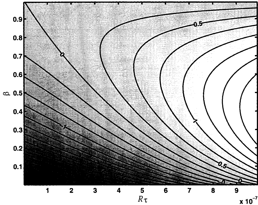
Figure 2.5: The change in the bulk isotopic content of an idealized mass of snow in units of permil after one year for a range of \beta (fraction of vapor leaving the firn) and R\tau (fraction of firn sublimated in time \tau ). Contour interval is 0.25 ‰. Our models show that it is possible to either enrich or deplete heavy isotopes in the firn. Additional environmental information at a site, such as the temperature of the firn as a function of depth and time of year, make it possible to use this model to predict the pattern of post-depositional change.
