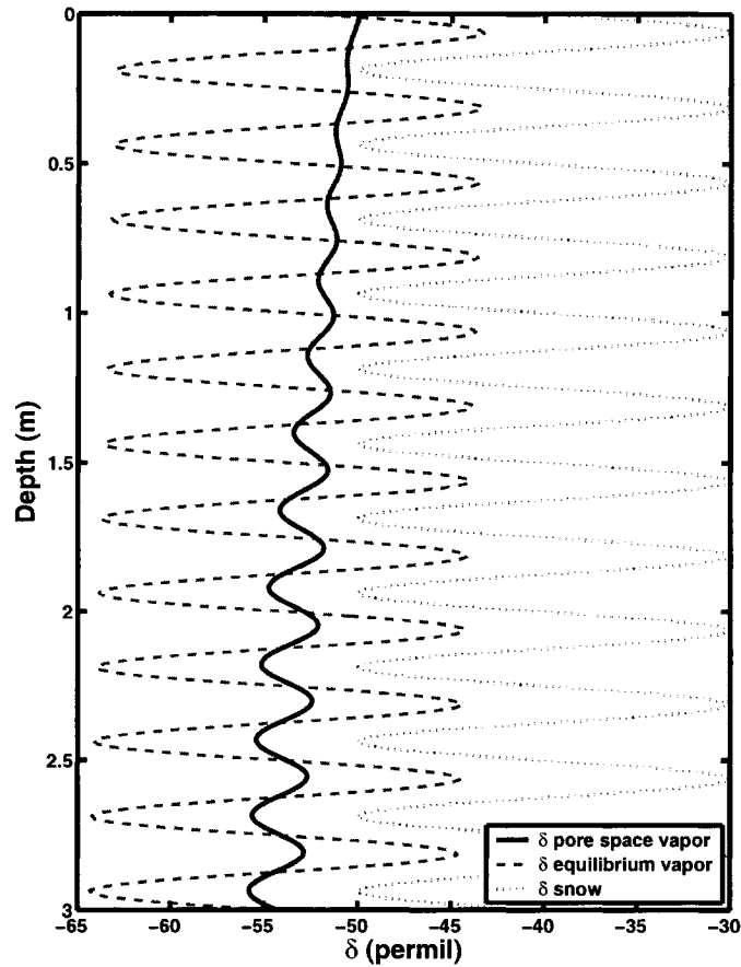
Figure 4.9: Numerical model prediction of pore-space vapor ( \delta_v , solid line), snow ( \delta_i , dotted line), and equilibrium vapor (from Equation (4.5), dashed line) during summer in regions of air outflow. The increase in the mean \delta_v value between 3 m and 2 m is due to the temperature sensitivity of the fractionation coefficient \alpha (Majoube, 1971). Above 2 m, the sublimation of surrounding snow grains (Fig. 4.4) becomes important. I assume that snow grains sublimate without fractionation. Consequently, sublimation of relatively heavy snow grains accelerates the increase in \delta_v . The gradual decrease in amplitude towards the surface is due to increased air flow velocities near the surface, which act to smooth out large variations in \delta_v .
