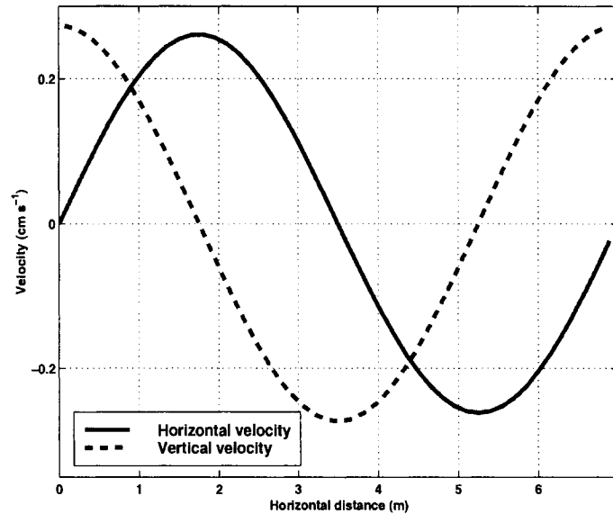
Figure 3.2: Near-surface air-flow velocities for \lambda = 7 m, h = 17 cm, and 10-meter wind speed = 8.25 \text{ m s}^{-1} . Horizontal and vertical velocities were calculated following the method of Colbeck (1989) and Waddington and others (1996), as described in Section 3.3. Horizontal velocities are positive to the right; vertical velocities are positive down. The surface topography parameters ( \lambda and h ) were tuned to produce the same pressure drop (5 Pa) over surface bumps used by Albert (2002). Air flows into the firn (vertical velocity is positive) on the intervals x = 0:1.75 m and 5.25:7 m. Air flows out of the firn (vertical velocity is negative) between x = 1.75 and 5.25 m. Since I use a constant permeability, the magnitude of the velocities decrease exponentially with depth with an e-folding scale of \lambda/2\pi (Equation (3.5)).
