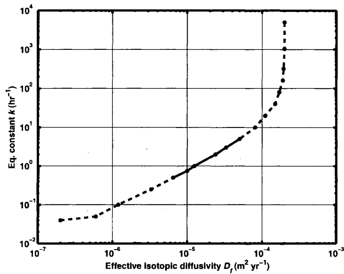
Figure 4.1: Effective isotopic diffusivity D_f ( \text{m}^2 \text{yr}^{-1} ) as a function of isotopic equilibration coefficient k ( \text{hr}^{-1} ). In this model run, firn temperature is uniform ( = -30^\circ \text{C} ), \rho_{\text{snow}} = 600 \text{ kg m}^{-3} , air-flow velocities in the firn are set to zero, and exchange as a result of vapor density gradients are neglected (i.e. no condensation or sublimation). Although the value of k between snow and water vapor is uncertain, I expect 0.1 \leq k \leq 5 \text{ hr}^{-1} ; this range is indicated with the solid line.
