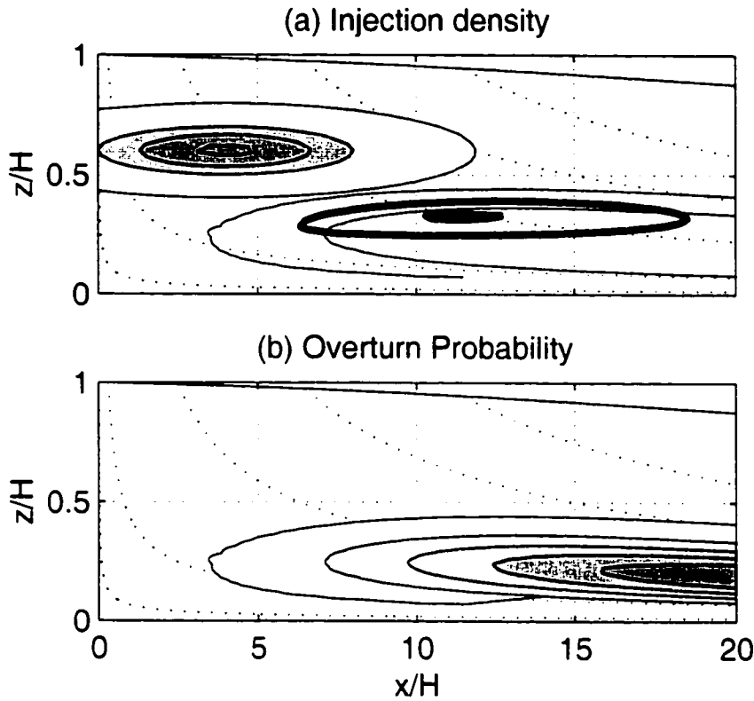
Figure 2.12: Overturn probability for binormal injection density in x and z coordinates. p(\theta, \mathbf{x}) = g(\theta)f(x)f(z) . Panel (a) also has contours ( heavy lines ) where the probability of observing an overturned segment in the 90 - 160^\circ range is largest.
