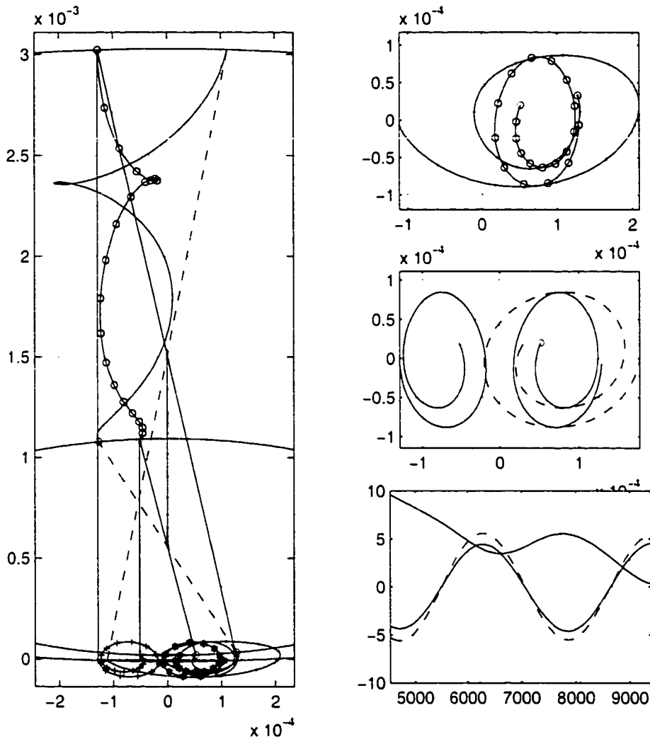
Figure F.4: Rotation and strain rates along a portion of a path (starting at (500m, 1000m)) over a sine bed.
