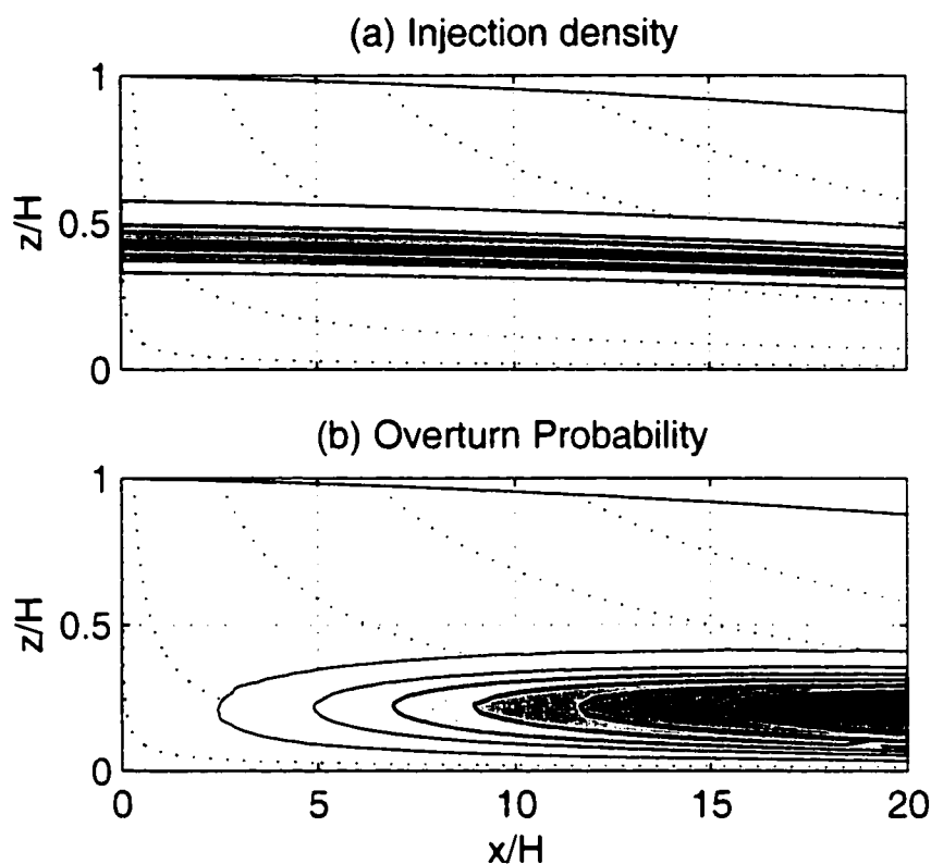
Figure 2.11: (a) Contours of an injection density, f(t) , that is Gaussian in travel time. These contours are aligned with isochrones. (b) Contours of the overturn probability, Q(90^\circ, \tau) . The pattern is similar to fixed injection time case plotted in Figure 2.9. Contour levels are not the same in the two panels.
