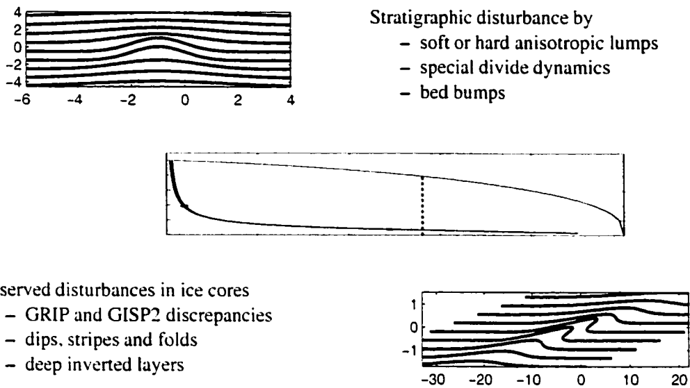
Figure 0.1: Large-scale flow deforms open disturbances into recumbent folds
