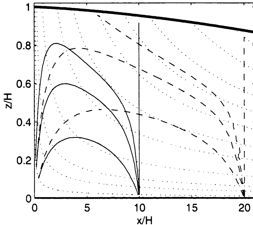
Figure 1.9: Precore slope angle contours ( \theta_f = 10^\circ, 30^\circ, \& 50^\circ ) for two core locations, 10H (solid lines) and 20H (dashed lines). The gray line marks where \theta_r = \theta_f .
