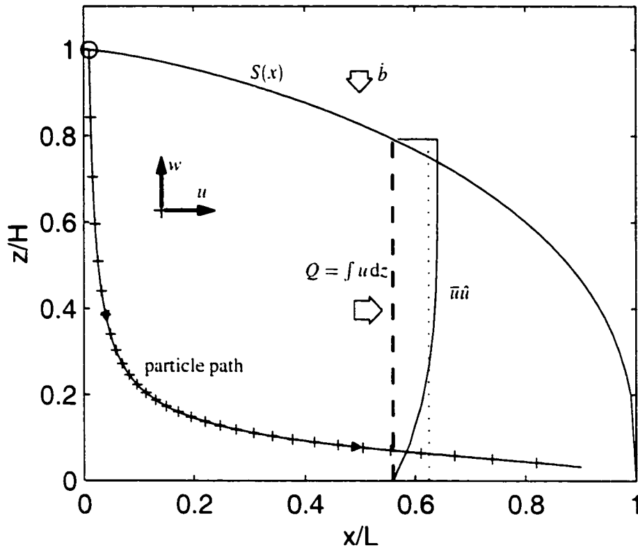
Figure 1.5: Flowband geometry and notation.
