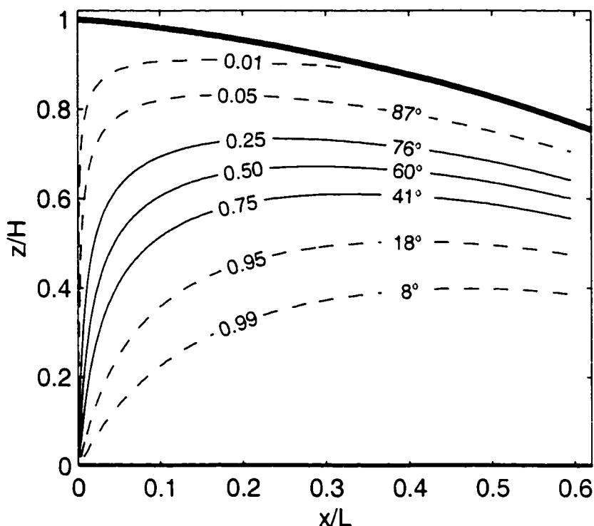
Figure 1.2: The kinematic vorticity number, W_k , and the critical wobble angle, \theta_r , for a simple ice sheet model. The left hand number on each contour, W_k , is a measure of the relative magnitudes of pure and simple shear. Pure shear dominates near the surface and under the divide ( W_k close to 0) while simple shear dominates elsewhere ( W_k close to 1). The right hand number, \theta_r is the segment angle that is not rotating at this point in the flow ( \cos^{-1} W_k ).
