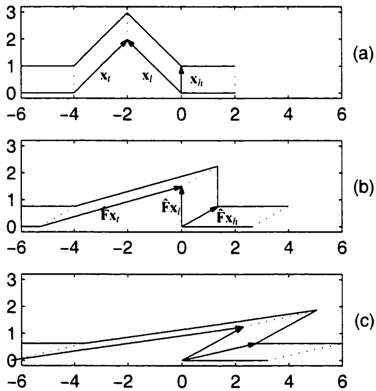
Figure 4.3: Overturning of a parallelogram disturbance. (a) Initial symmetric disturbance. (b) Leading edge becomes vertical. (c) Overturned fold.
