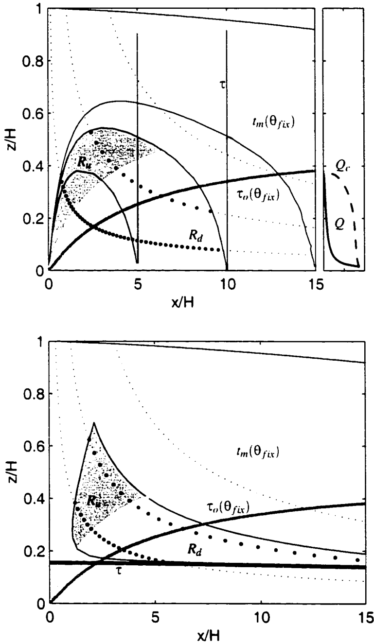
Figure 2.10: (upper) The R_u and R_d regions for observation points along a vertical core. Their boundaries lie on the \theta_f = \theta_{fix} precore angle contour.
