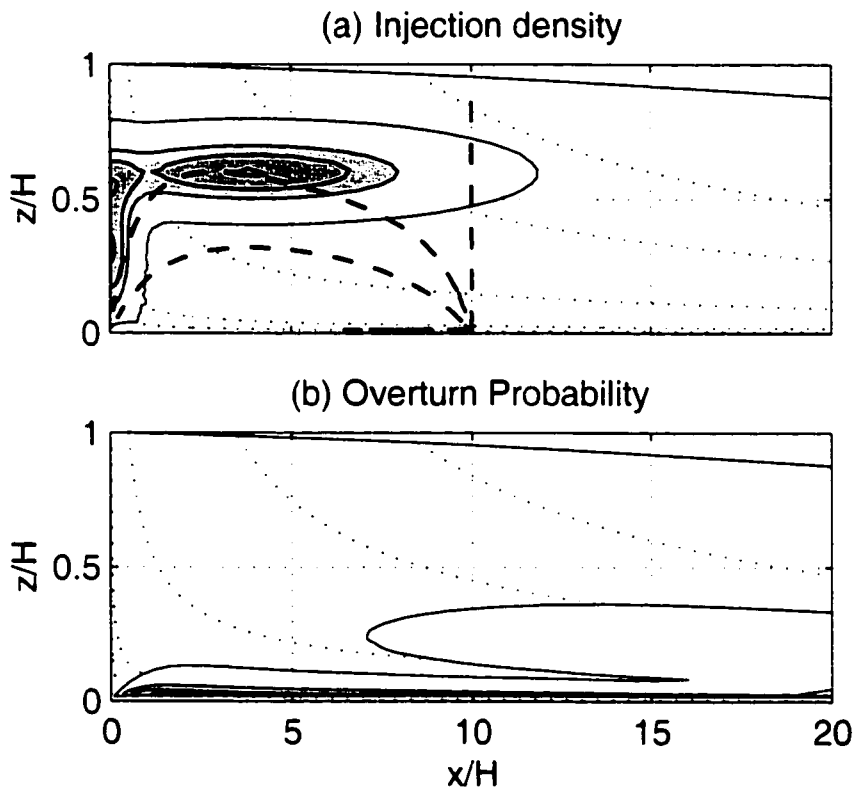
Figure 2.14: Overturn probability for a two zone injection density. The injection pattern in (a) is the combination of the patterns from Figure 2.12 and Figure 2.13. Panel (a) includes the 10 and 30° precore contours (dashed) from Figure 2.2. The 30° contour cuts across the upper injection region, while the 10° contour crosses a portion of the divide region.
