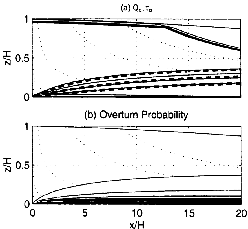
Figure C.3: Uniform injection density in time as in Figure 2.15. (a) Contours of Q_c (shaded); \tau_o contours (heavy dashed lines). (b) Q(90^\circ) contours (shaded)
