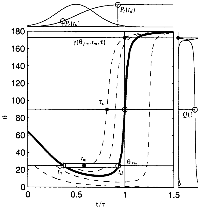
Figure 2.6: Known injection angle ( \theta_{fix} = 25^\circ ), probabilistic injection time. (top) The injection density f(t) (shaded) and the injection distribution P_i(t) versus t . (right) The corresponding observation distribution Q(\phi) (line) and density q(\phi) (shaded). The circles on the two panels mark the terms in Q(90^\circ) = P_i(t_d) - P_i(t_u) . (center) The injection region that contributes to Q(90^\circ) is the gray bar between the t_u and t_d points on the \theta_f(t, \tau) curve. A segment injected at t_m is the first one to overturn (at time \tau_0 ).
