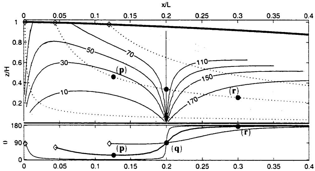
Figure 1.8: The upper plot shows contours of the precore angles, \theta_f , in degrees. The lower plot shows these angles along selected particle paths (marked with \diamond at the surface). (p), (q), and (r) points in Figure 1.7 are also shown.
