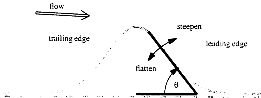
Figure 1.4: Prototypical disturbance, illustrating our notation, including leading edge , trailing edge , and \theta . Segment slope is measured relative to horizontal (pointing upstream). Not shown is the slight slope (relative to horizontal) of the undisturbed stratigraphy. One could imagine a disturbance such as this forming around a rheologically stiffer 'lump' in the ice. Such a lump would also disturb the layers below it.
