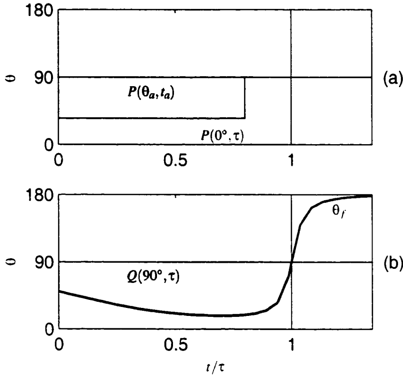
Figure 2.3: Integration areas for P(\theta_a, t_a) and Q(90^\circ, \tau) . (a) P(\theta_a, t_a) can be obtained by integrating p(\theta, t) over the rectangle defined by 0 \leq t \leq t_a and \theta_a \leq \theta \leq 90^\circ . (b) Q(90^\circ, \tau) is obtained by integrating p(\theta, t) over the area bounded by \theta_f(t, \tau) . This is a subset of the area covered by P(0^\circ, \tau) (which equals Q(0^\circ, \tau) ).
