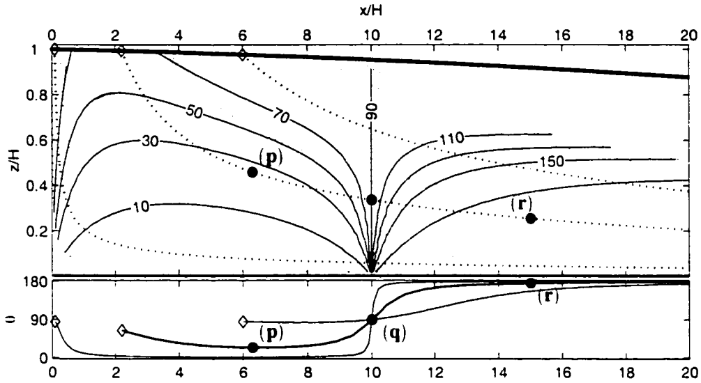
Figure 2.2: (upper) Particle paths ( dotted ) and contours of \theta_f(t, t_c) , the precore slope angle in degrees, plotted along the inner portion of an ice sheet flowband. The ice divide is on the left ( x/H = 0 ). (lower) \theta_f(t, t_c) along selected particle paths (marked with \diamond at the surface). Corresponding points on both panels are marked (p), (q), (r). The values of \theta_f at these points are 24^\circ , 90^\circ , and 176^\circ .
