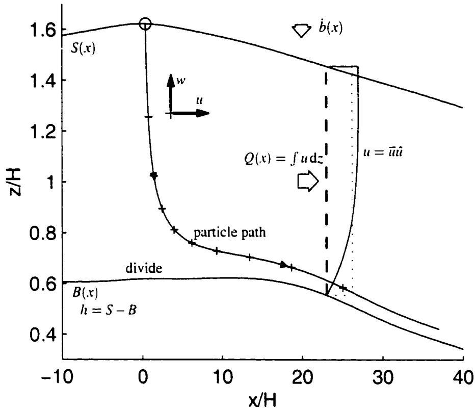
Figure A.1: Flowband geometry and notation.
