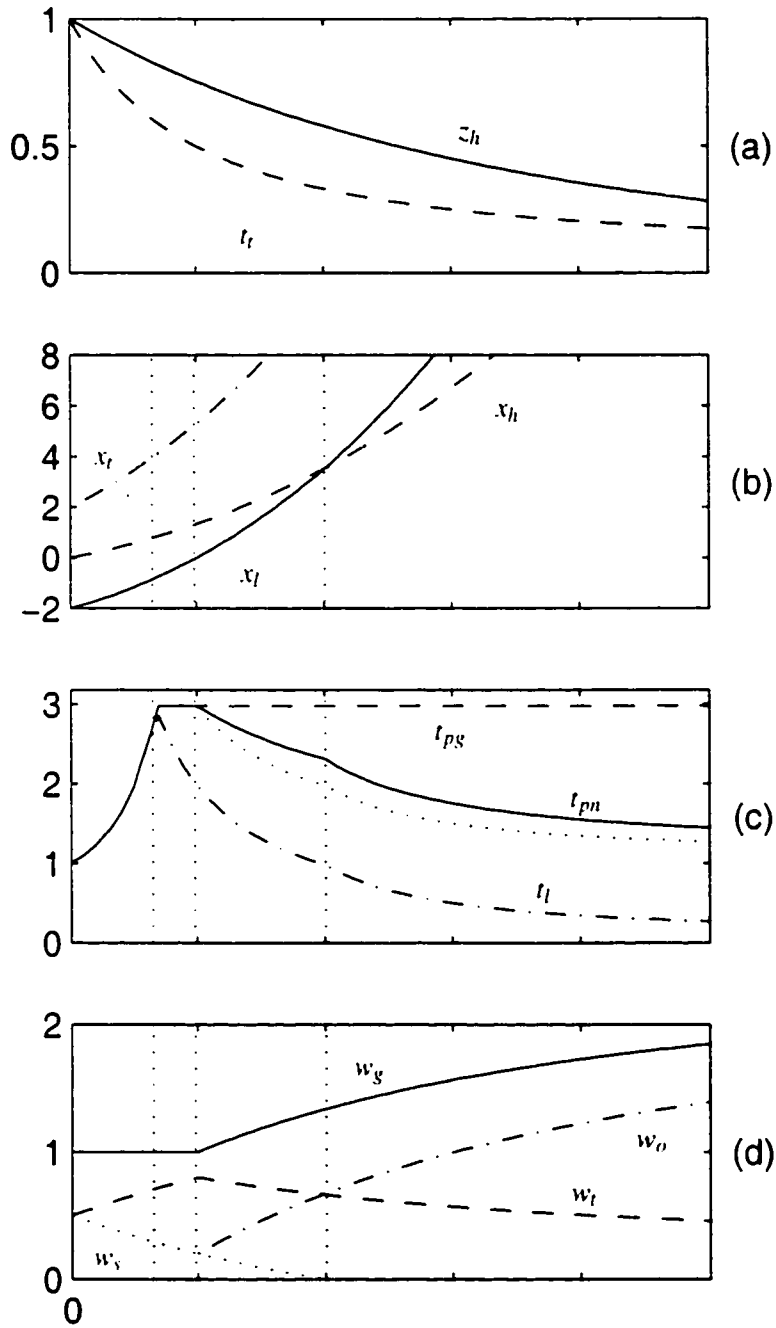
Figure 4.4: Thicknesses and widths at selected points on a disturbance through time (horizontal axis).
