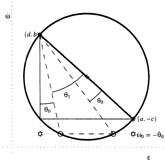
Figure E.2: Mohr circle for calculating the angle, \theta_1 , that is not rotating with respect to the surface isochrone, \theta_0 . \dot{\epsilon} and \dot{\omega} of the \theta_0 and \theta_1 segments are plotted as circles near the bottom of the Mohr circle. The inscribed right triangle illustrates the equation (E.24) for \theta_0 + \theta_1 . The hexagonal points outside the Mohr circle can be used with equation (E.23) to give \tan \theta_0 + \tan \theta_1 .
