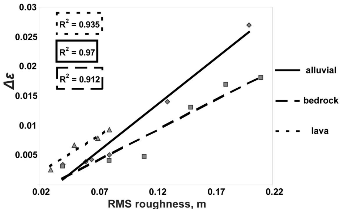
Figure 9. Effect of surface RMS on \Delta\epsilon in alluvial, bedrock, and lava flow surfaces. Value of \epsilon used for the model calculations in all cases was 0.9. All surfaces were isothermal at 300K.
